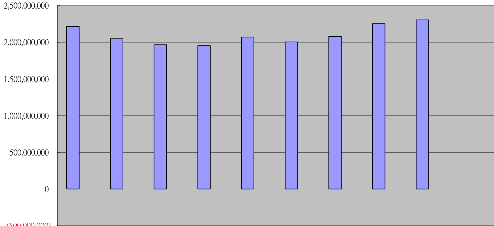
Taiwan Taoyuan International statistics (Freight)2010~2018
